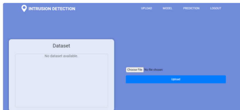
Fig 5.2.5 Upload Page
